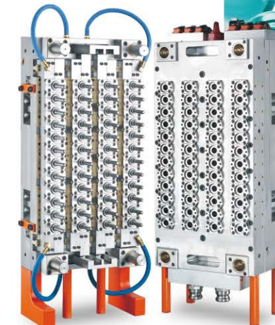
48-cavity Preform Mould
