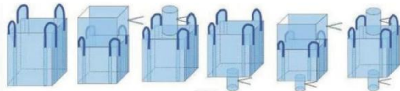
ST-FIBC007 OPEN TOP AND FLAT BOTTOM ST-FIBC008 DUFFLE TOP AND FLAT BOTTOM ST-FIBC009 FILLING SPOUT AND FLAT BOTTOM ST-FIBC010 OPEN TOP AND DISCHARGE SPOUT ST-FIBC011 DUFFLE TOP AND DISCHARGE SPOUT ST-FIBC012 FILLING SPOUT AND DISCHARGE SPOUT
